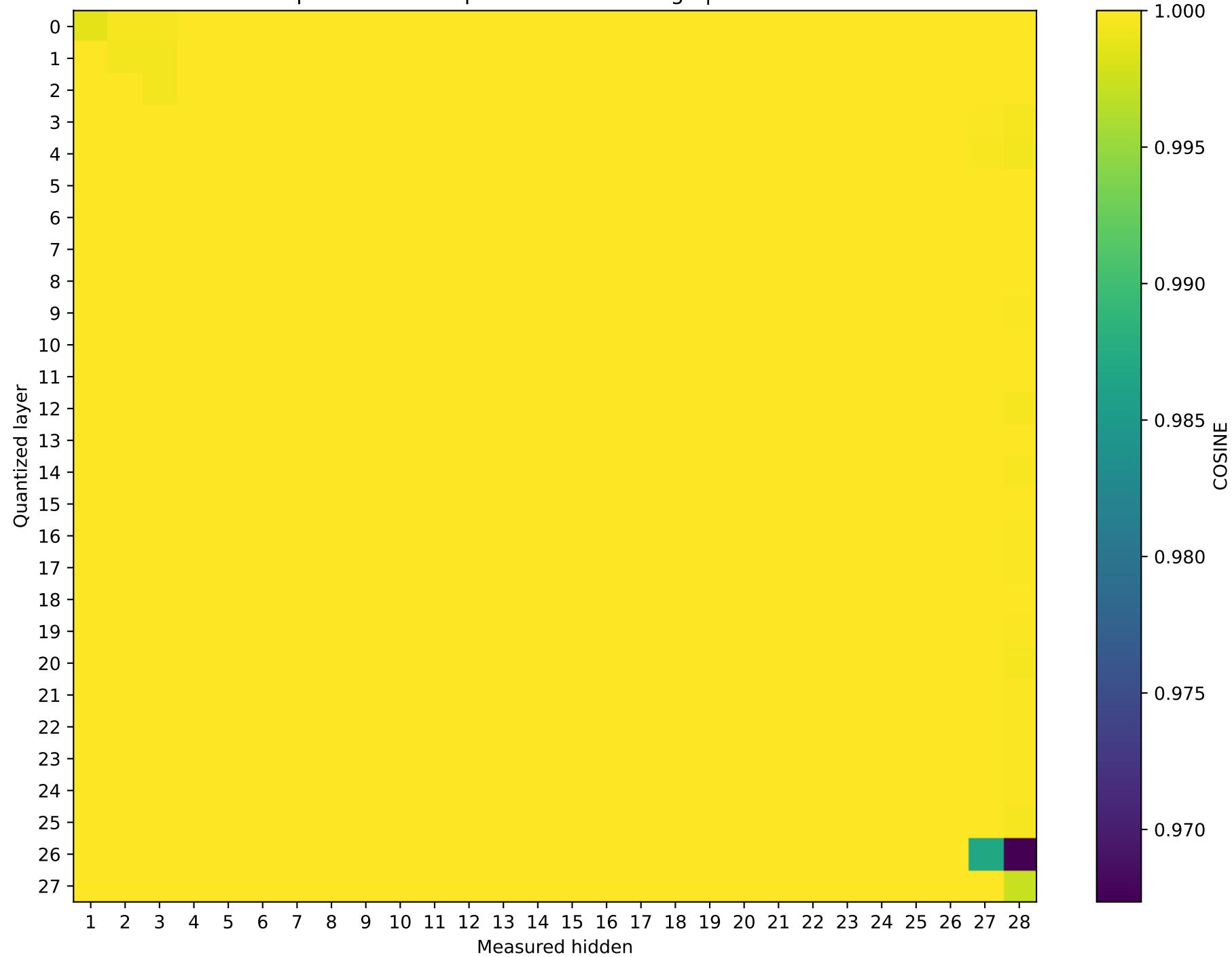
Qwen2.5-7B-Instruct Prompt 4: cos sim representation damage | float32 → int8
