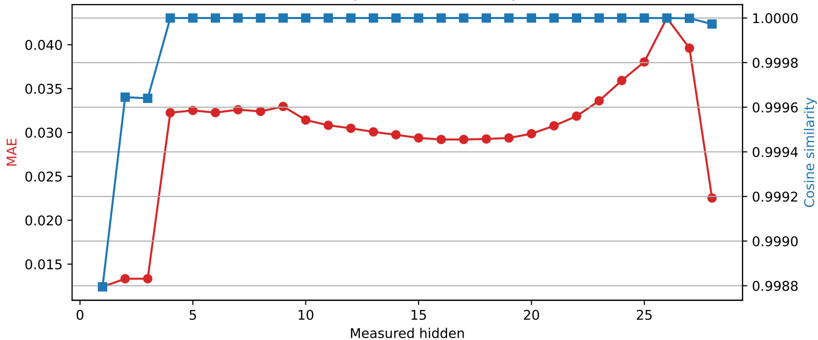
Qwen2.5-7B-Instruct | Quantized layer 0 | float64 → int8
