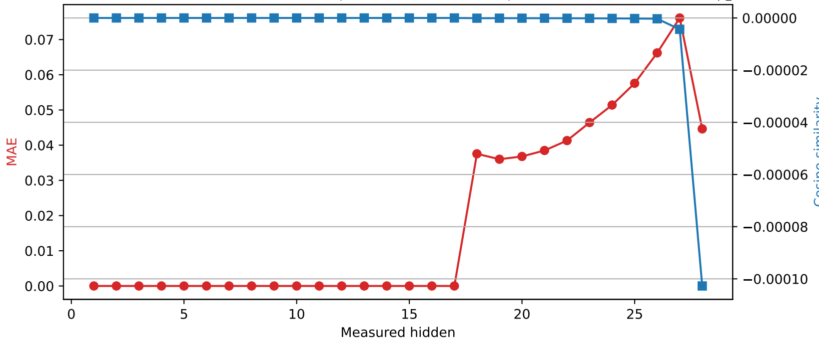
Qwen2.5-7B-Instruct | Quantized layer 17 | float64 → int8
