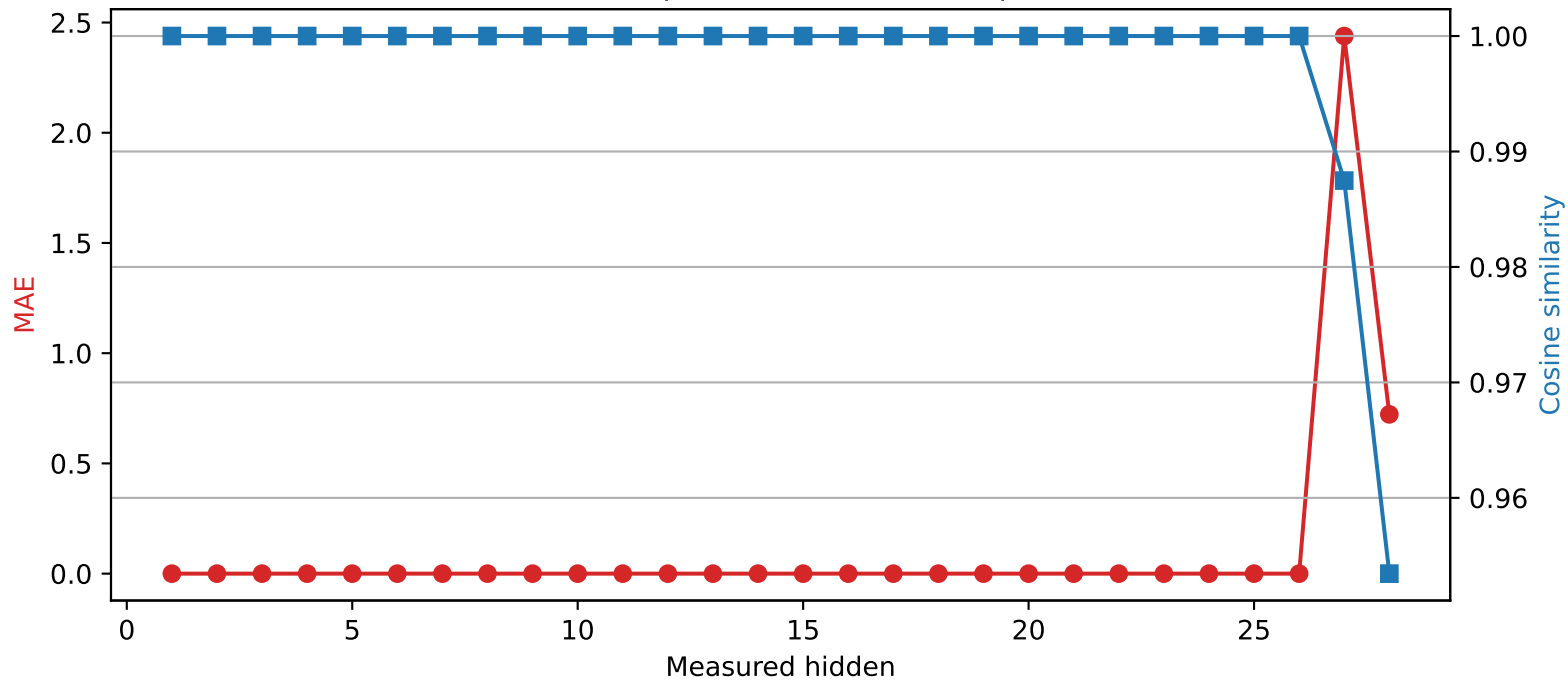
Qwen2.5-7B-Instruct | Quantized layer 26 | float64 → int8
