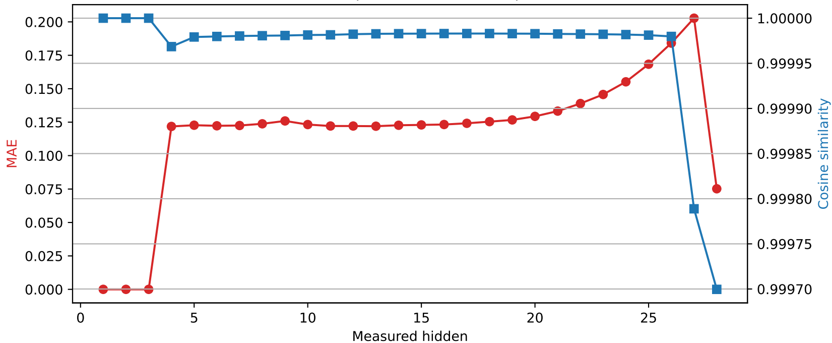
Qwen2.5-7B-Instruct | Quantized layer 3 | float64 → int8
