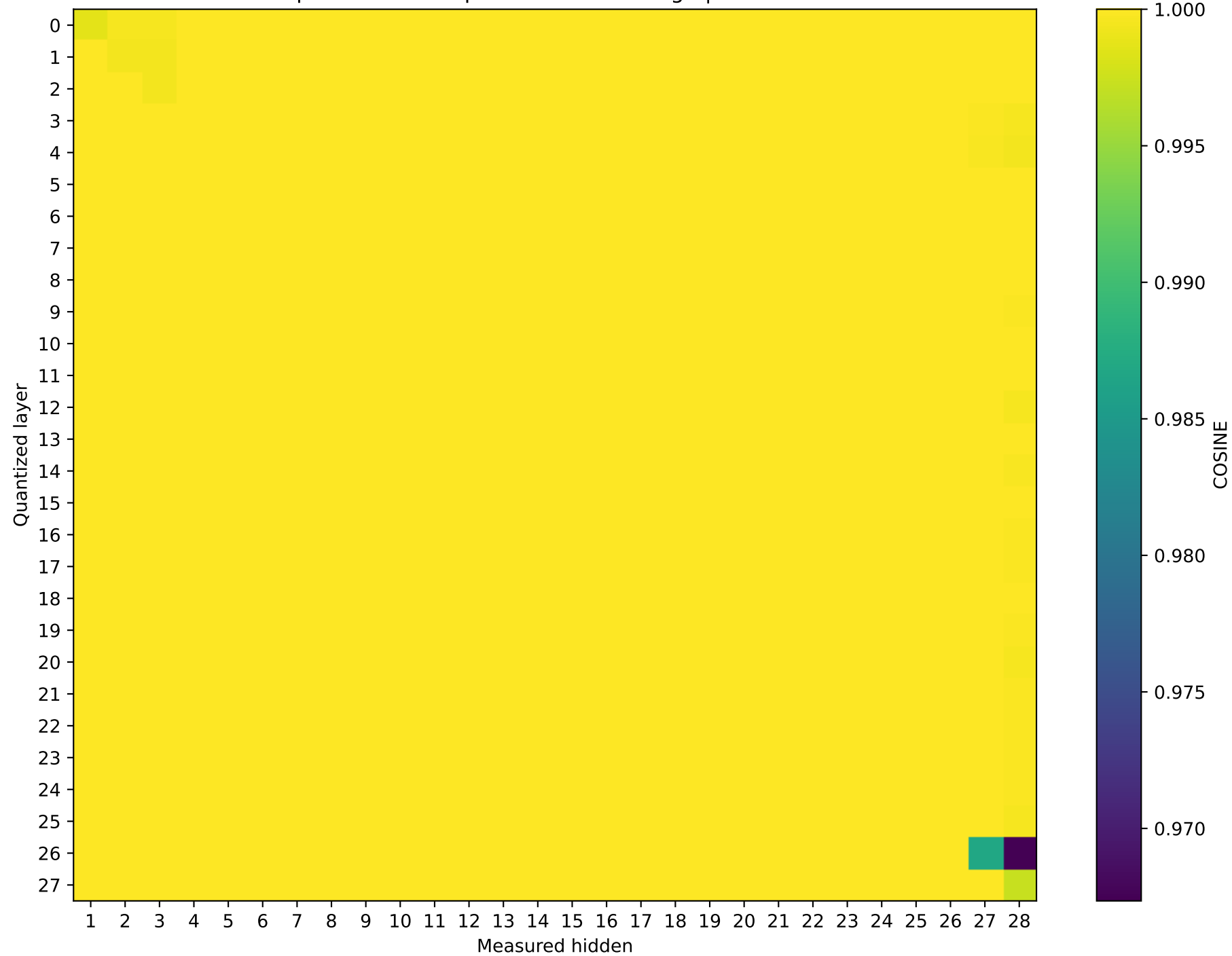
Prompt 4: cos sim representation damage | float64 → int8
