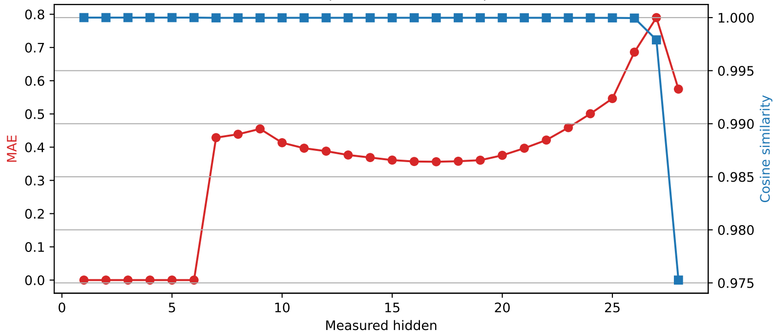
Qwen2.5-7B-Instruct | Quantized layer 6 | float16 \rightarrow int4
