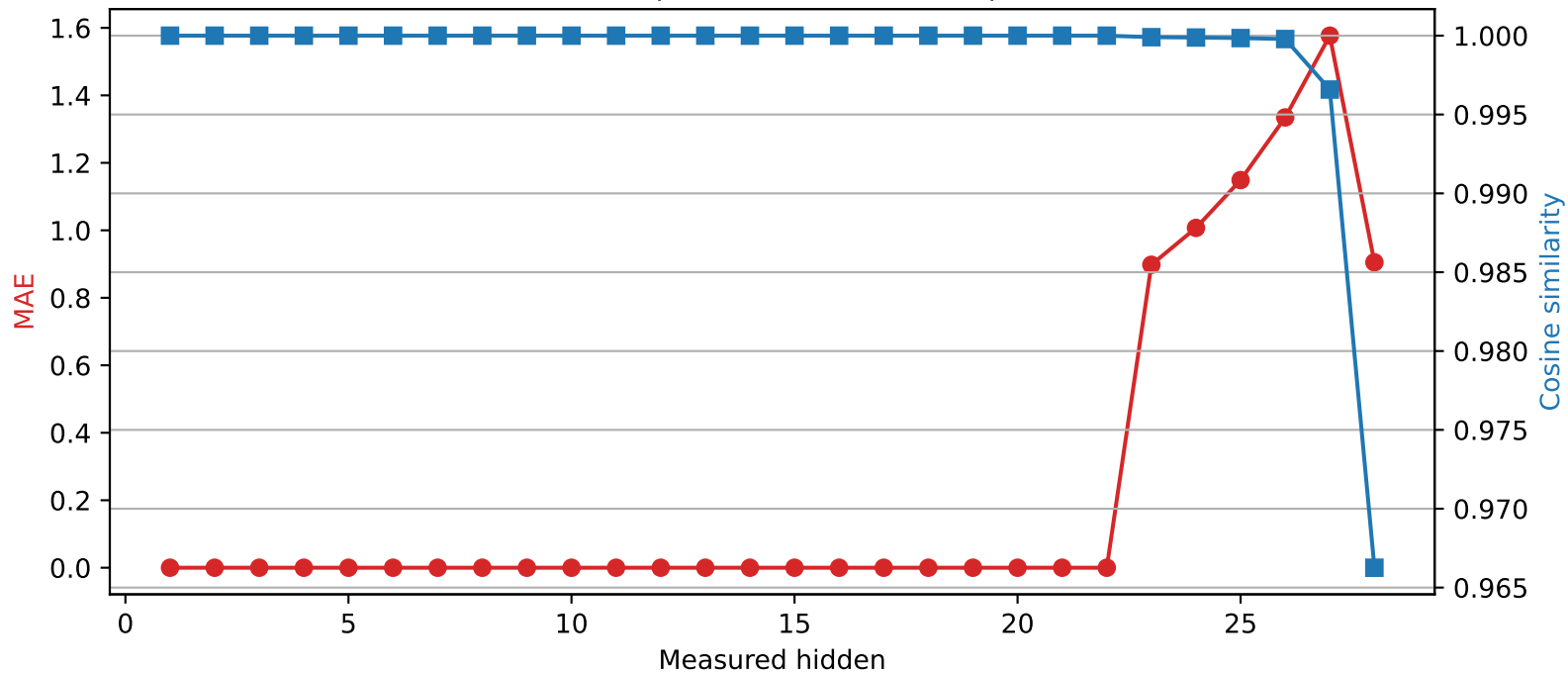
Qwen2.5-7B-Instruct | Quantized layer 22 | float16 → int4
