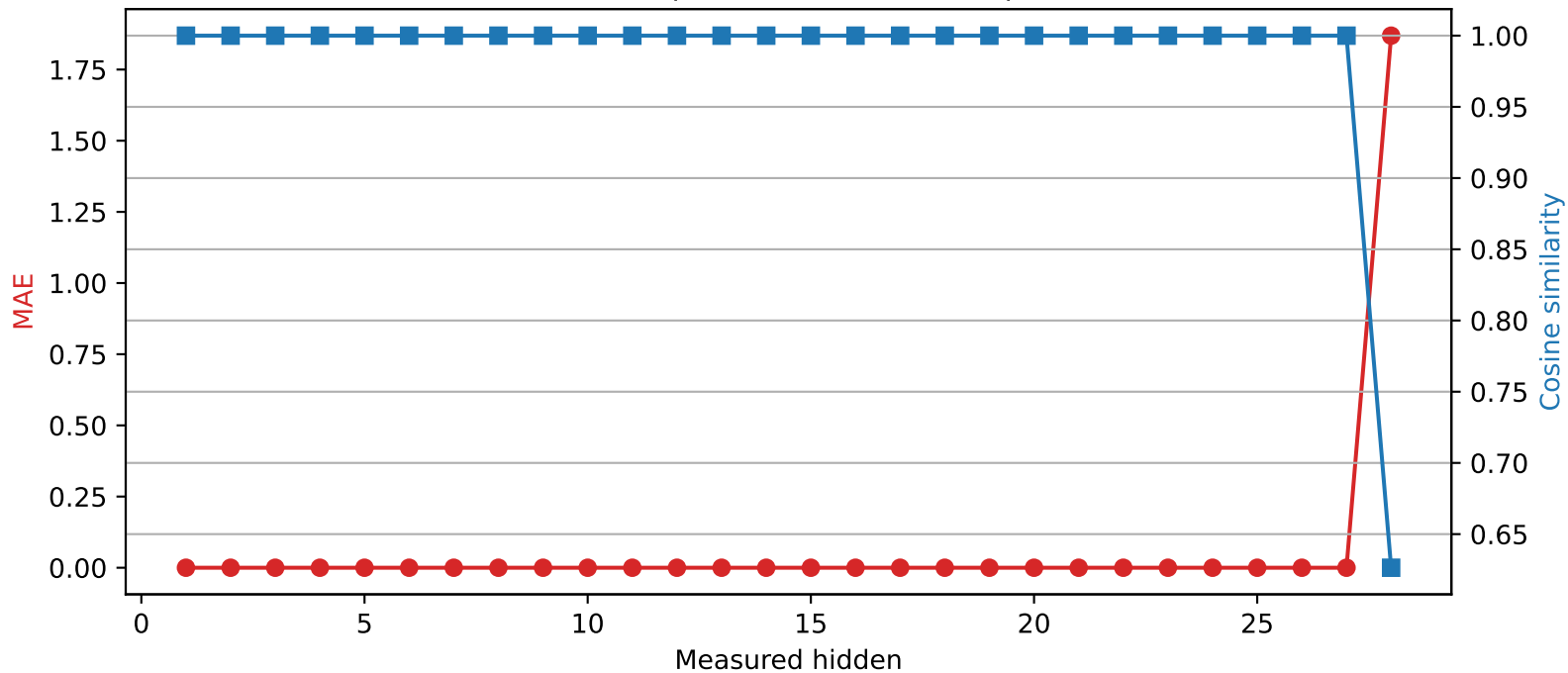
Qwen2.5-7B-Instruct | Quantized layer 27 | float16 → int4
