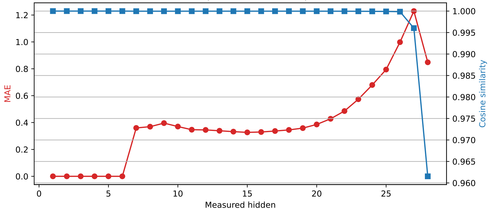
Qwen2.5-7B-Instruct | Quantized layer 6 | float16 → int4
