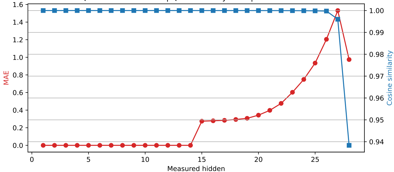
Qwen2.5-7B-Instruct | Quantized layer 14 | float16 \rightarrow int4
