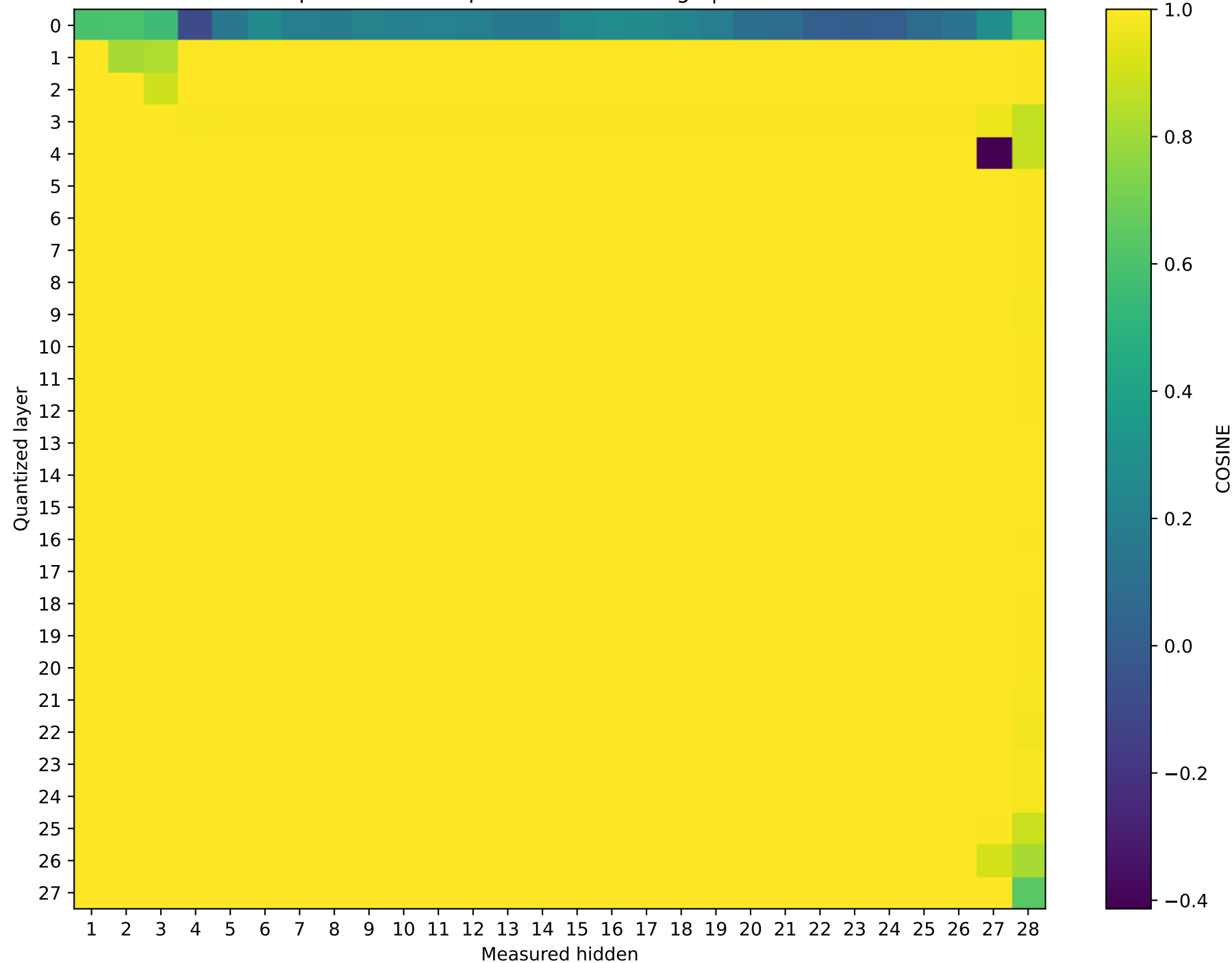
Qwen2.5-7B-Instruct Prompt 4: cos sim representation damage | float16 \rightarrow int4
