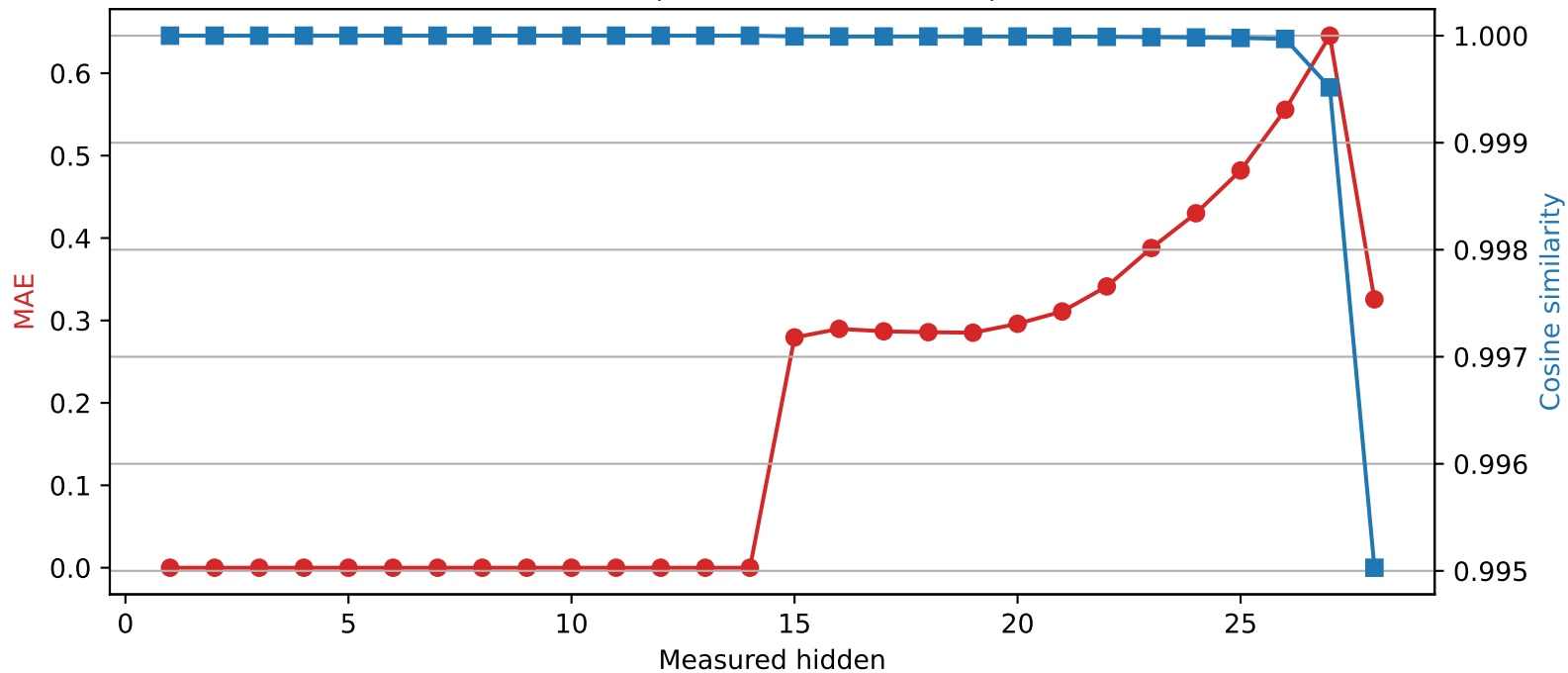
Qwen2.5-7B-Instruct | Quantized layer 14 | float16 → int4
