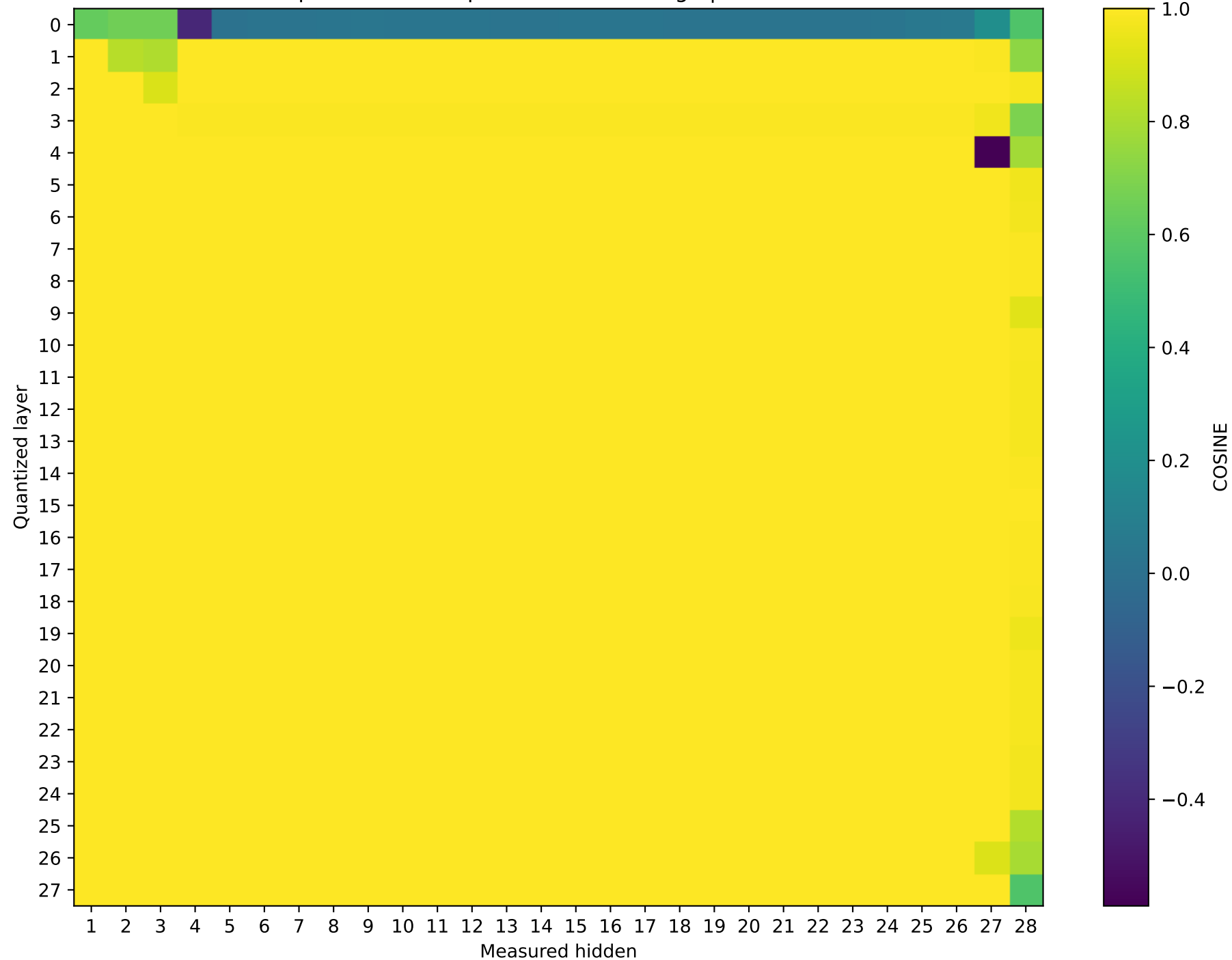
Qwen2.5-7B-Instruct Prompt 0: cos sim representation damage | float32 → int4
