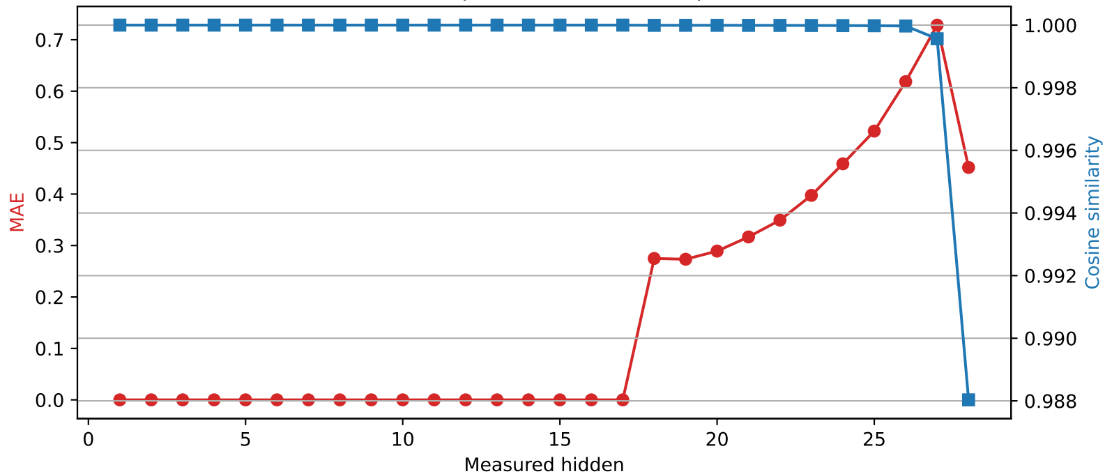
Qwen2.5-7B-Instruct | Quantized layer 17 | float32 → int4
