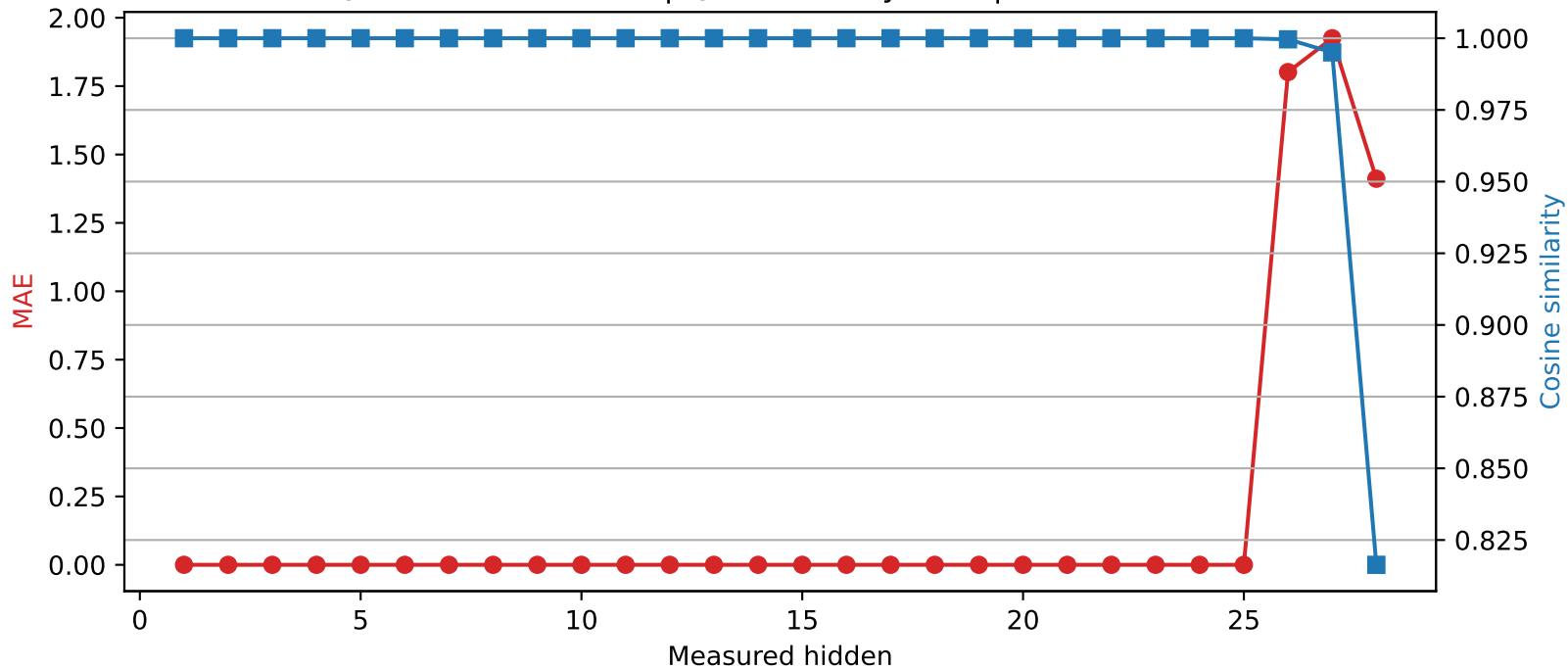
Qwen2.5-7B-Instruct | Quantized layer 25 | float32 \rightarrow int4
