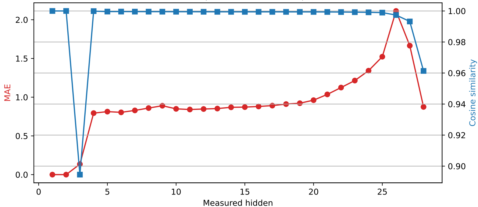
Qwen2.5-7B-Instruct | Quantized layer 2 | float32 → int4
