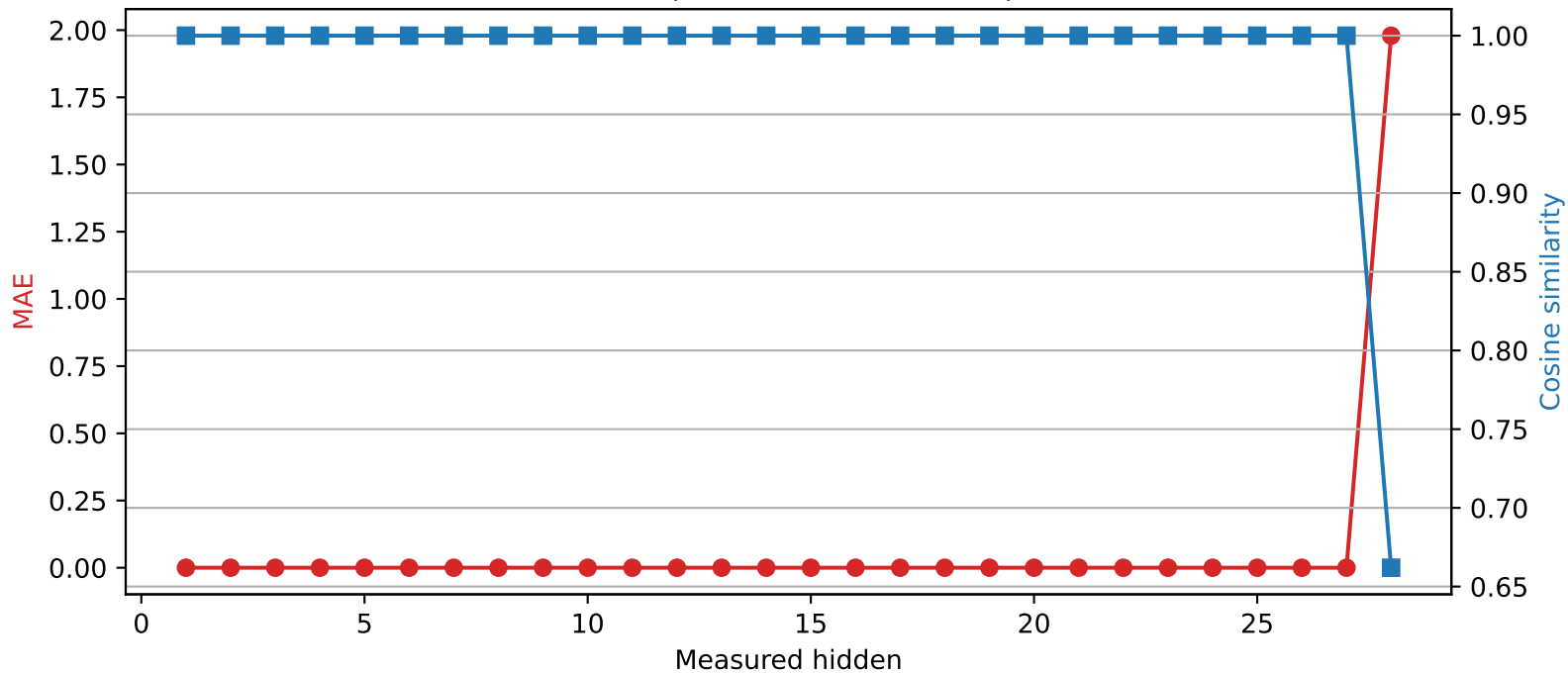
Qwen2.5-7B-Instruct | Quantized layer 27 | float32 \rightarrow int4
