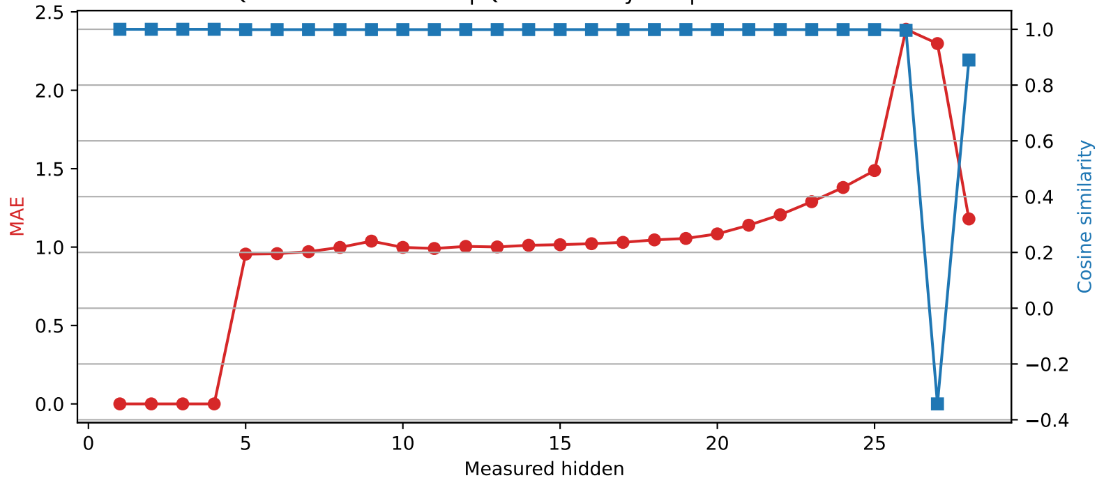
Qwen2.5-7B-Instruct | Quantized layer 4 | float32 → int4
