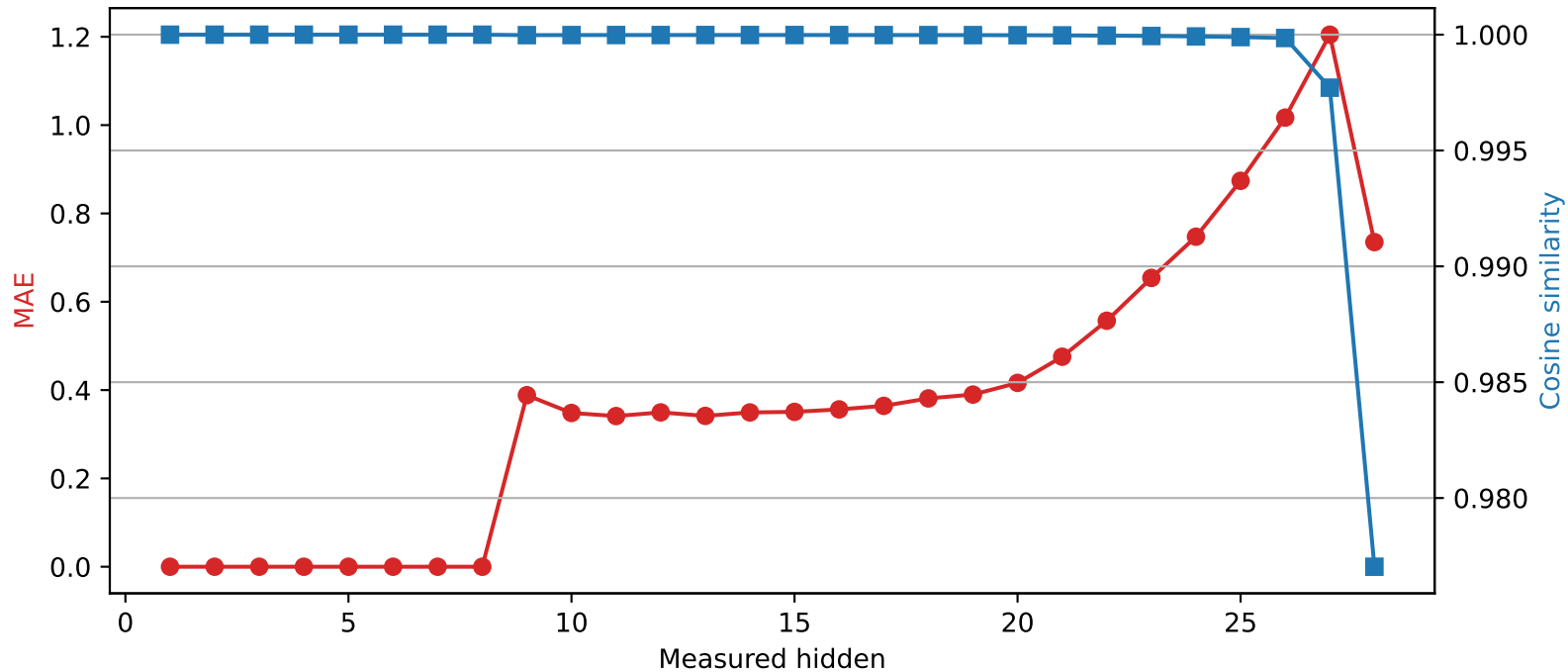
Qwen2.5-7B-Instruct | Quantized layer 8 | float32 \rightarrow int4
