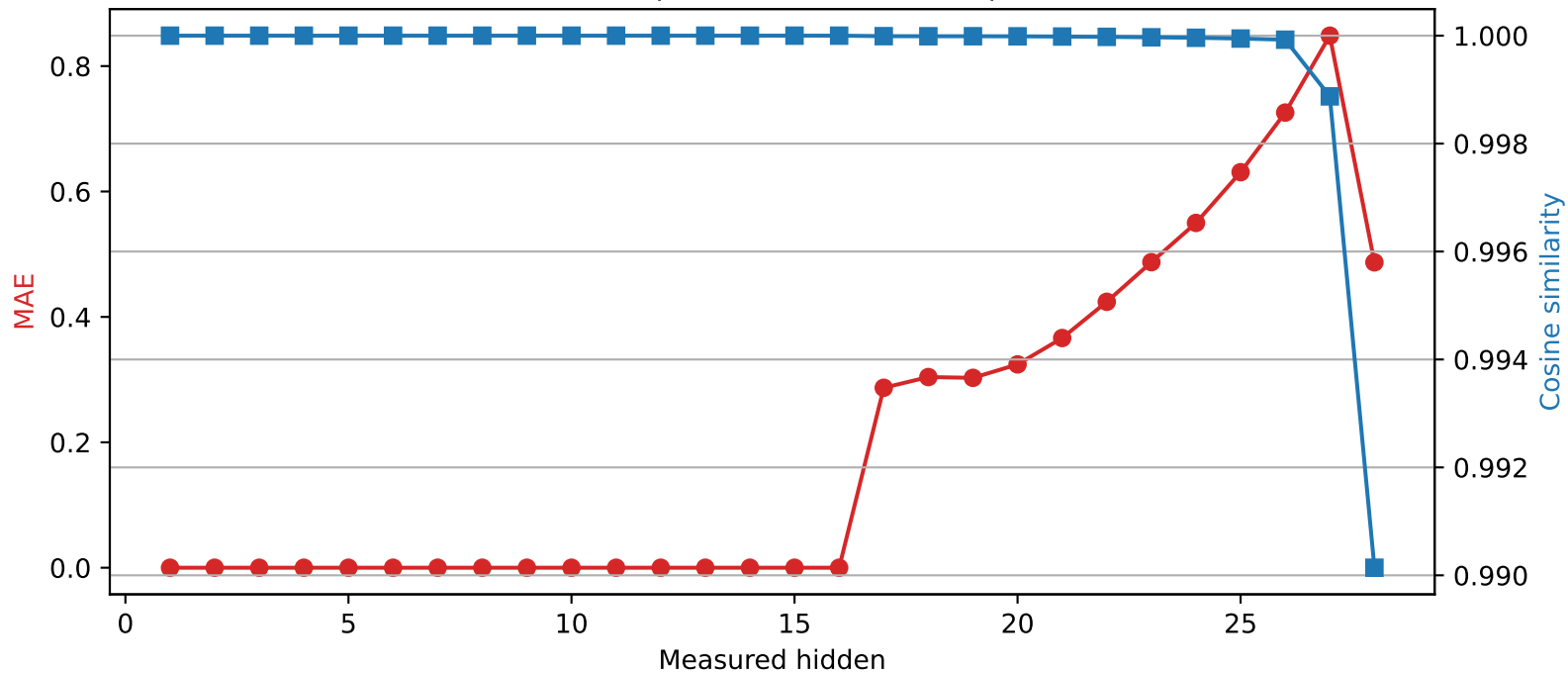
Qwen2.5-7B-Instruct | Quantized layer 16 | float32 \rightarrow int4
