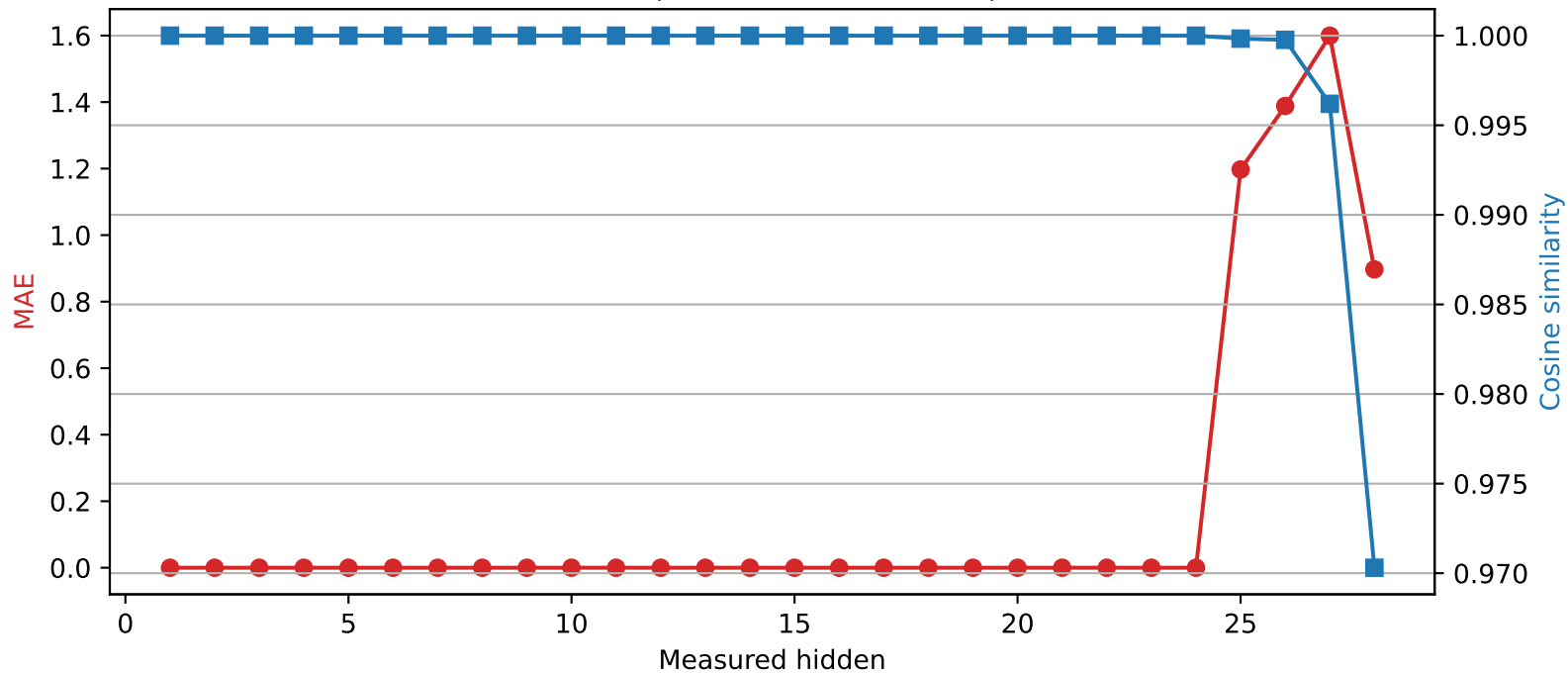
Qwen2.5-7B-Instruct | Quantized layer 24 | float32 → int4
