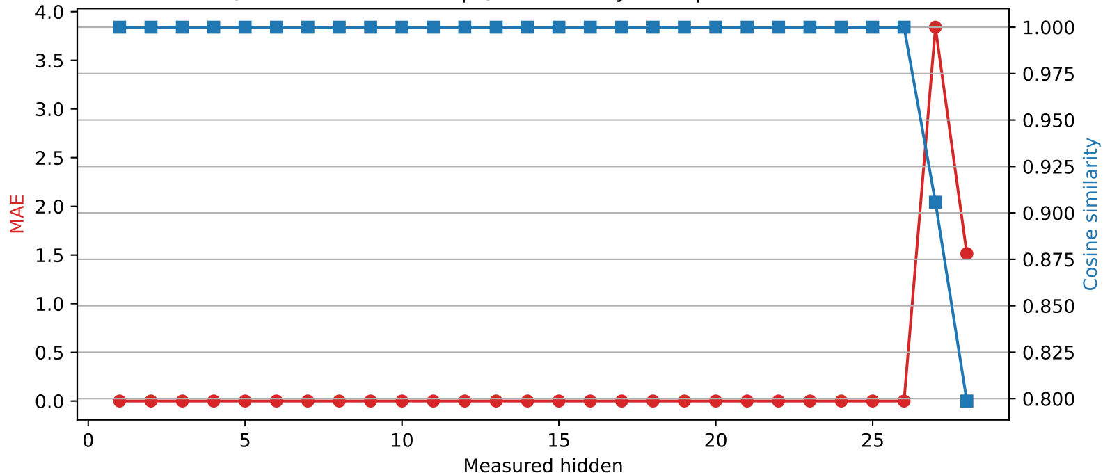
Qwen2.5-7B-Instruct | Quantized layer 26 | float32 → int4
