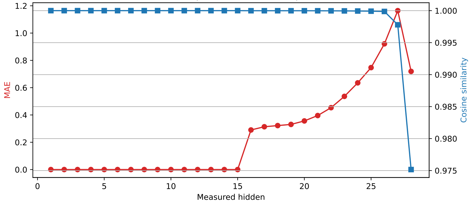
Qwen2.5-7B-Instruct | Quantized layer 15 | float32 → int4
