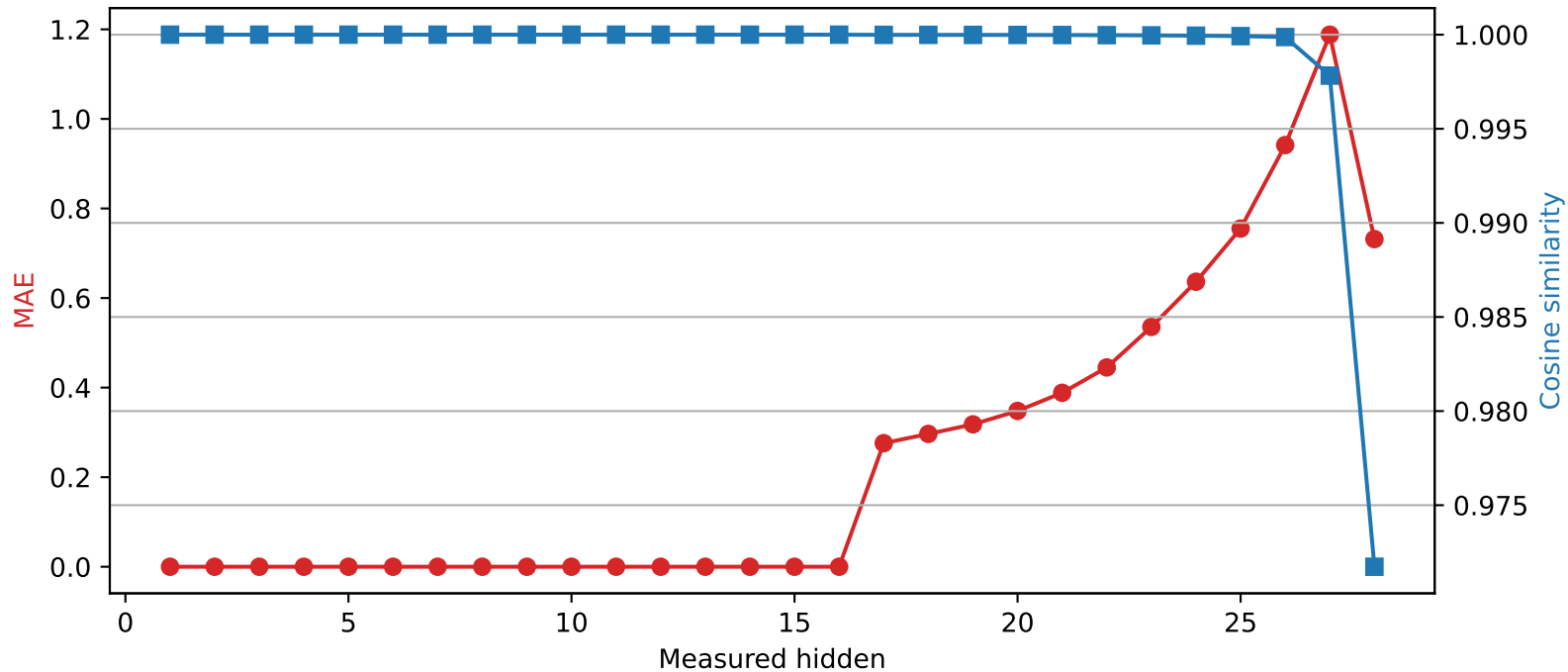
Qwen2.5-7B-Instruct | Quantized layer 16 | float32 → int4
