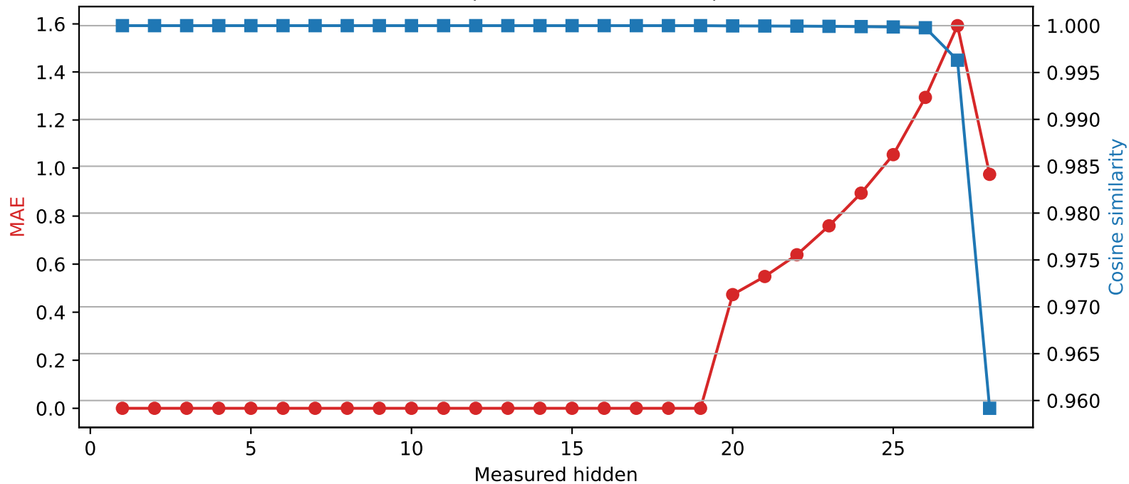
Qwen2.5-7B-Instruct | Quantized layer 19 | float32 → int4
