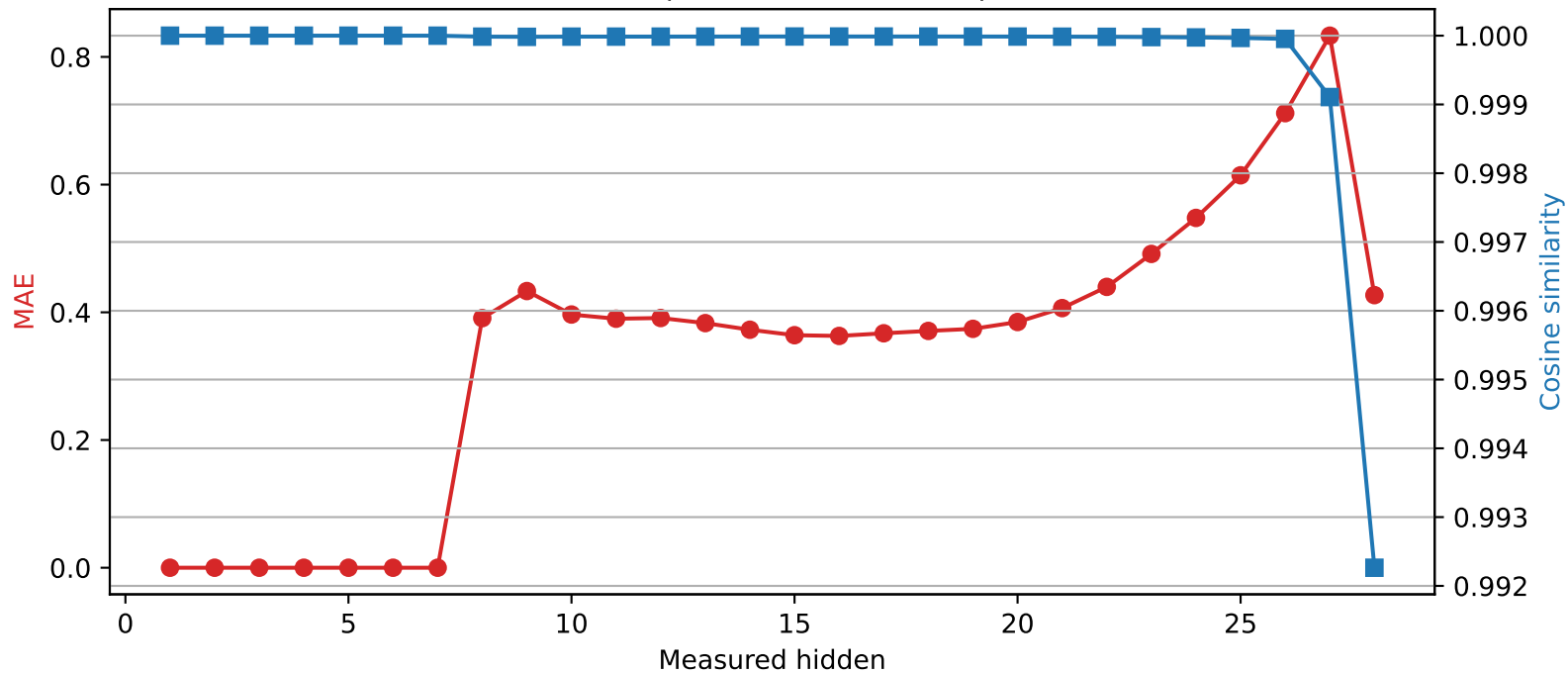
Qwen2.5-7B-Instruct | Quantized layer 7 | float32 → int4
