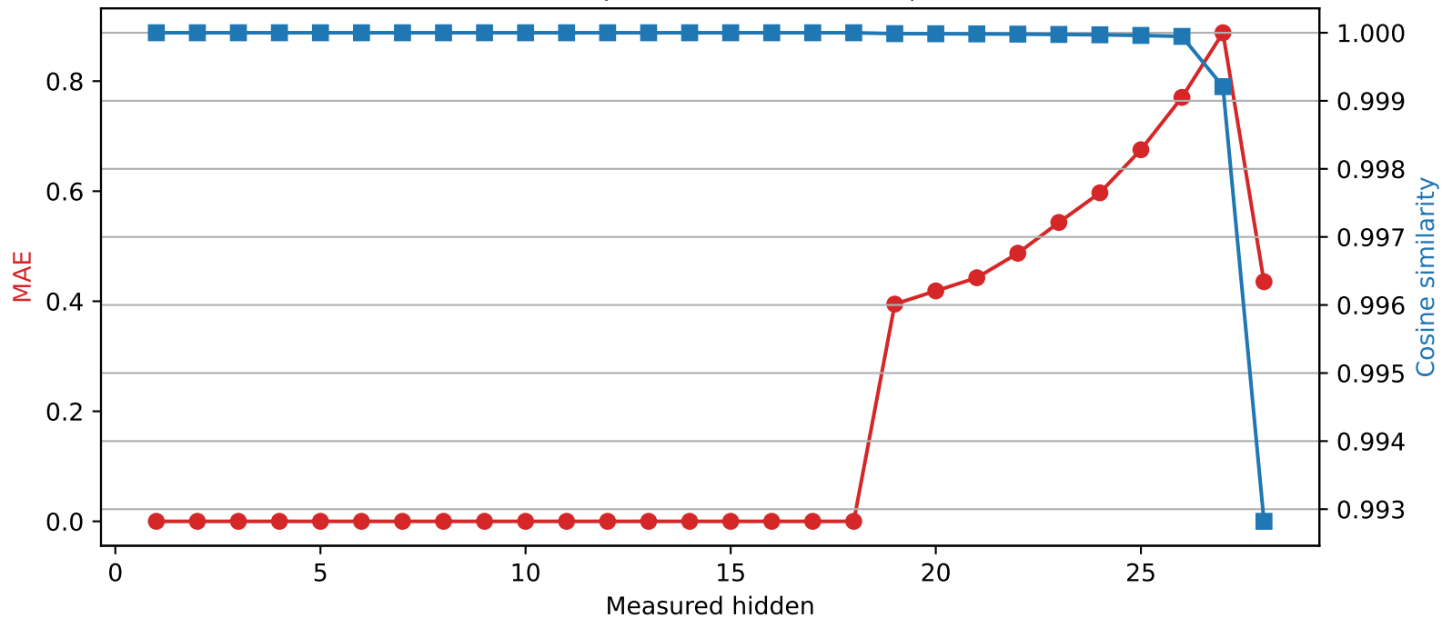
Qwen2.5-7B-Instruct | Quantized layer 18 | float32 → int4
