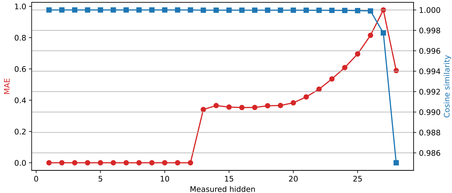
Qwen2.5-7B-Instruct | Quantized layer 12 | float64 → int4
