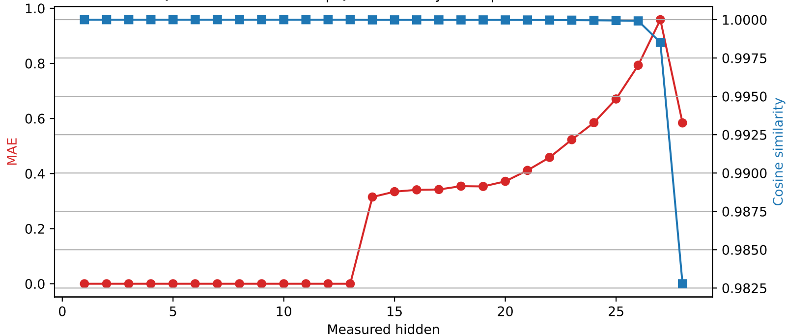
Qwen2.5-7B-Instruct | Quantized layer 13 | float64 → int4
