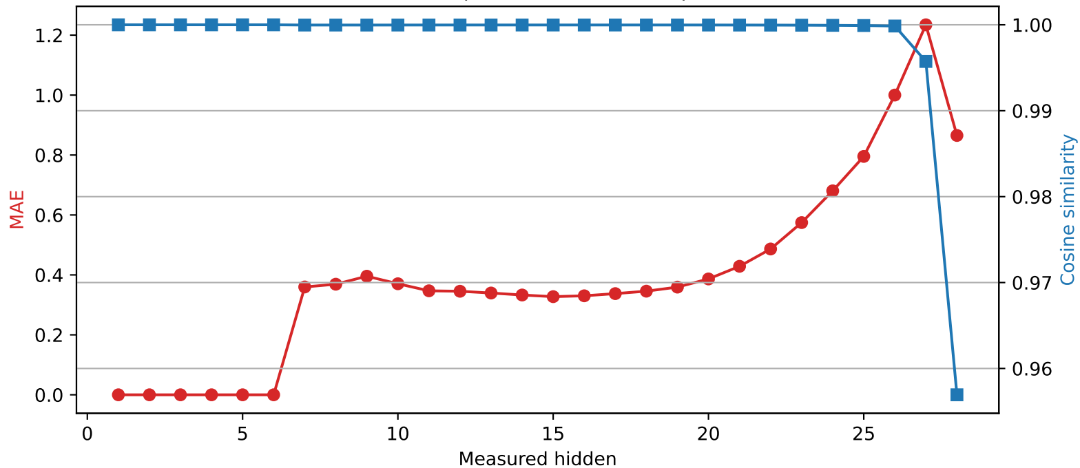
Qwen2.5-7B-Instruct | Quantized layer 6 | float64 → int4
