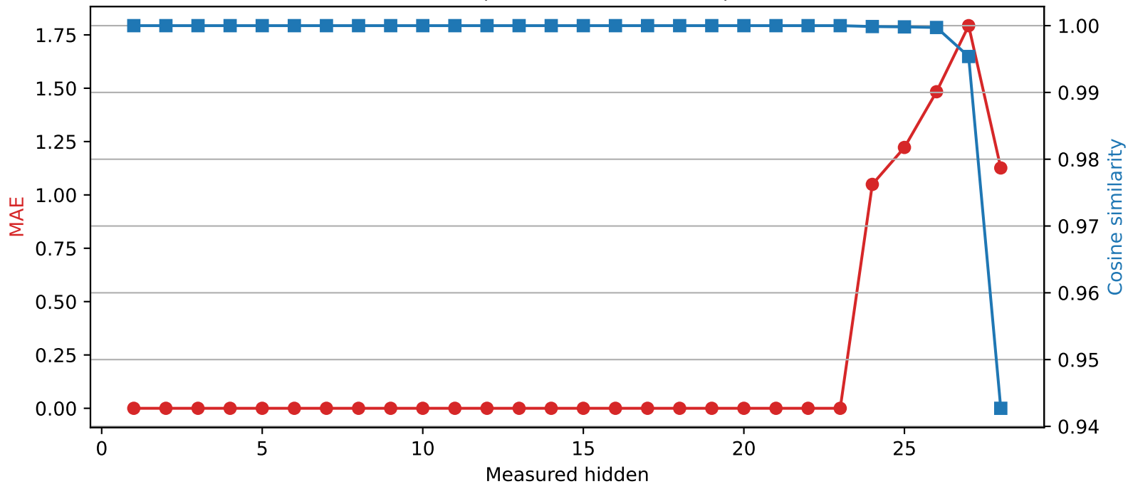
Qwen2.5-7B-Instruct | Quantized layer 23 | float64 \rightarrow int4
