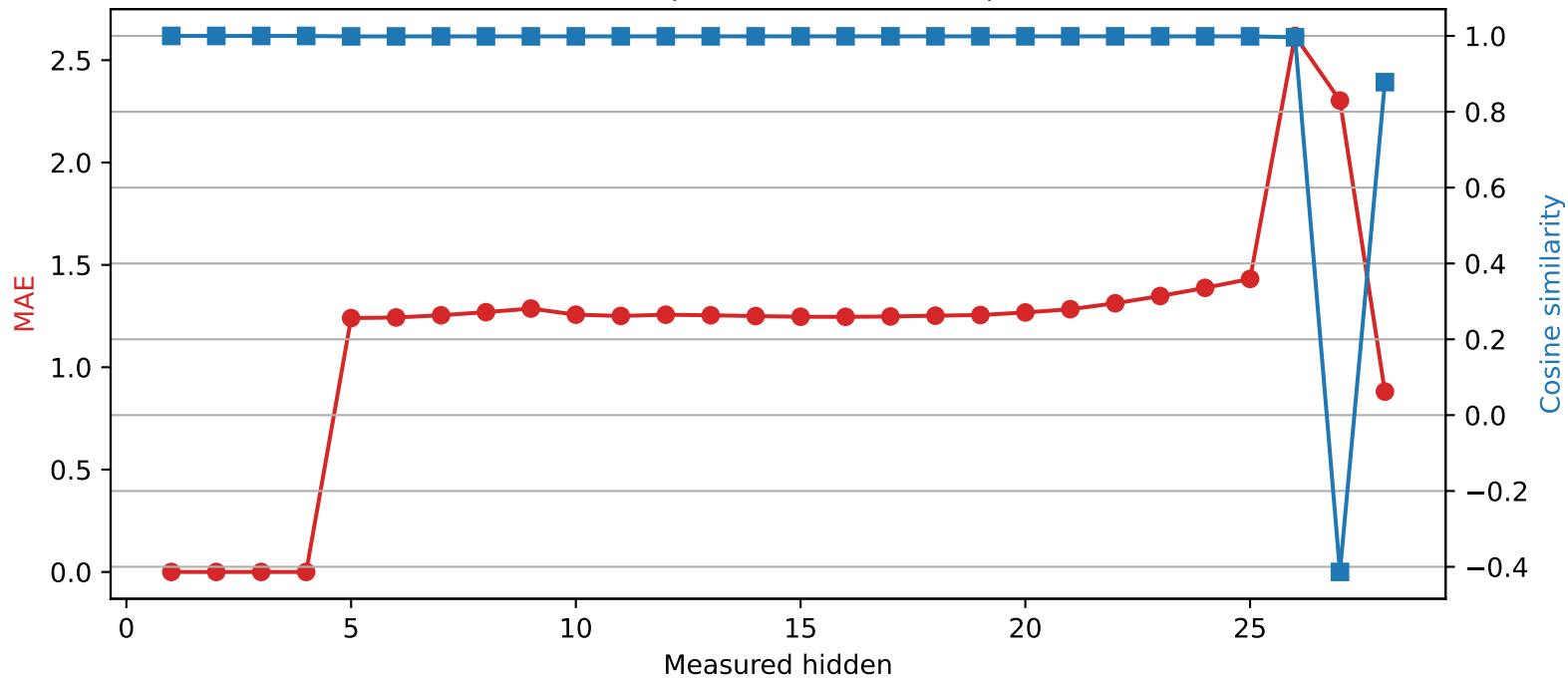
Qwen2.5-7B-Instruct | Quantized layer 4 | float64 → int4
