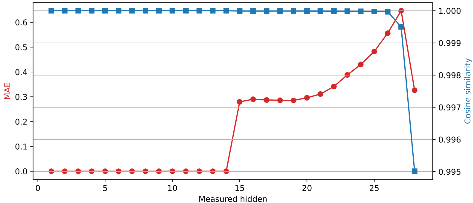
Qwen2.5-7B-Instruct | Quantized layer 14 | float64 → int4
