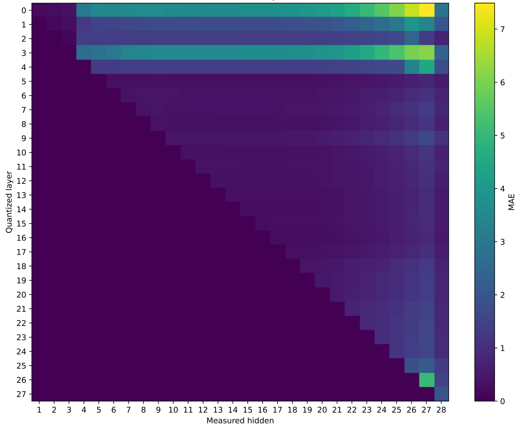
Model: Qwen2.5-7B-Instruct | float16 \rightarrow int2
