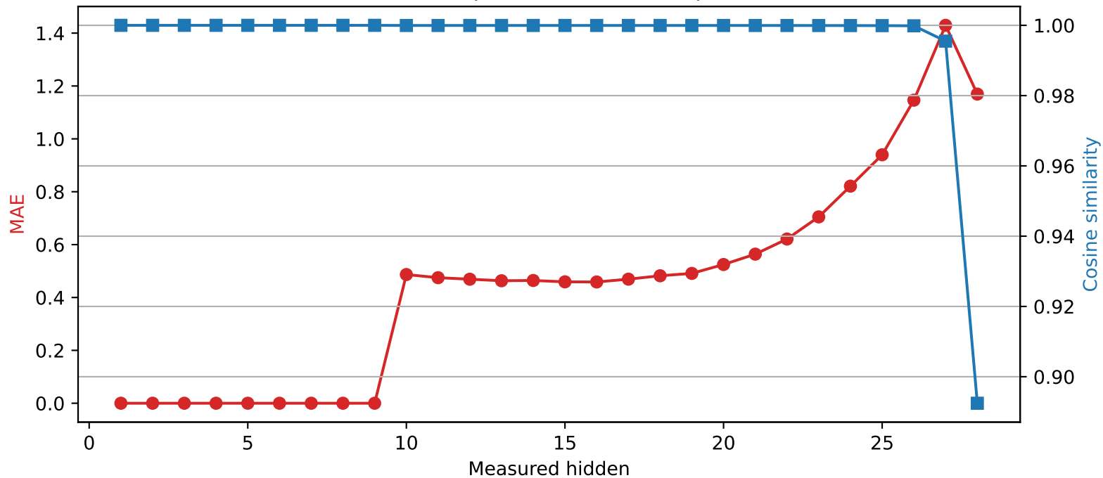
Qwen2.5-7B-Instruct | Quantized layer 9 | float16 \rightarrow int2
