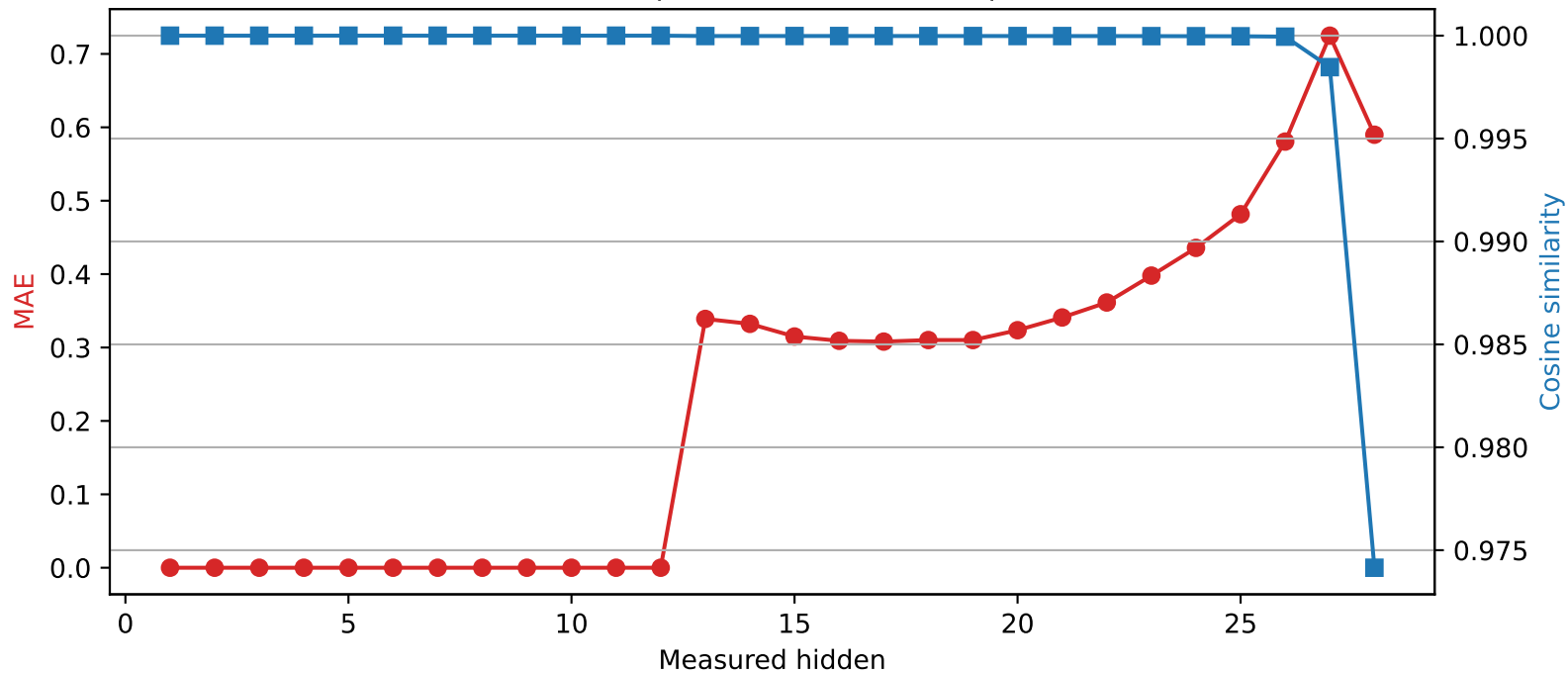
Qwen2.5-7B-Instruct | Quantized layer 12 | float16 → int2
