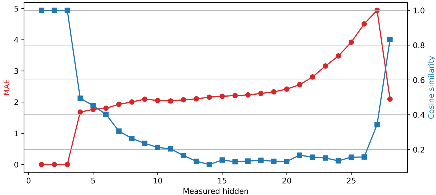
Qwen2.5-7B-Instruct | Quantized layer 3 | float16 \rightarrow int2
