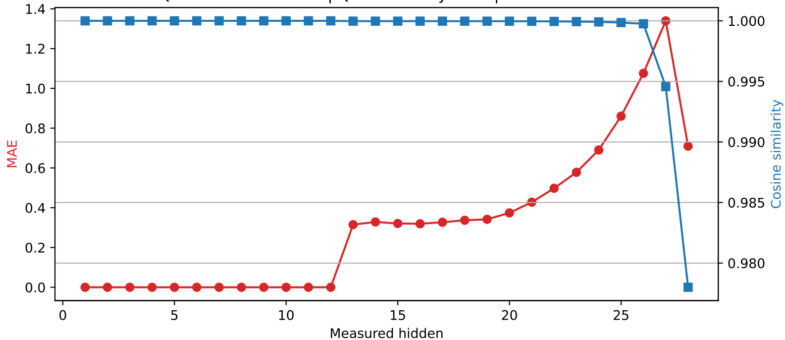
Qwen2.5-7B-Instruct | Quantized layer 12 | float16 \rightarrow int2
