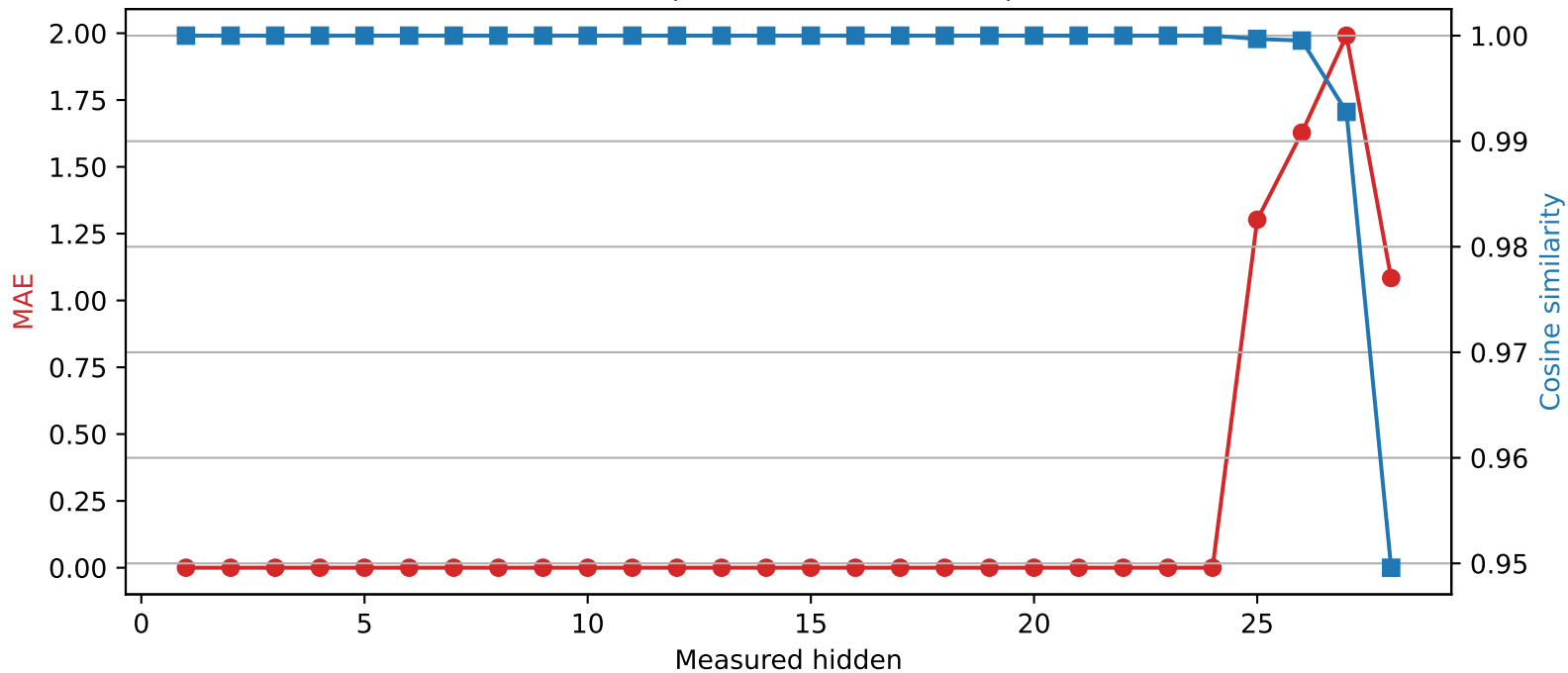
Qwen2.5-7B-Instruct | Quantized layer 24 | float16 → int2
