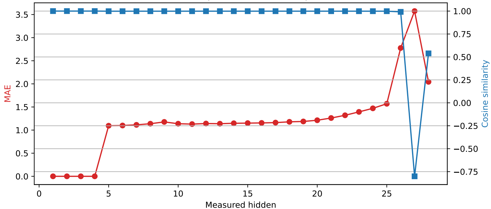
Qwen2.5-7B-Instruct | Quantized layer 4 | float16 \rightarrow int2
