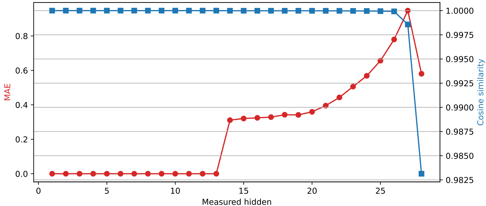
Qwen2.5-7B-Instruct | Quantized layer 13 | float16 → int2
