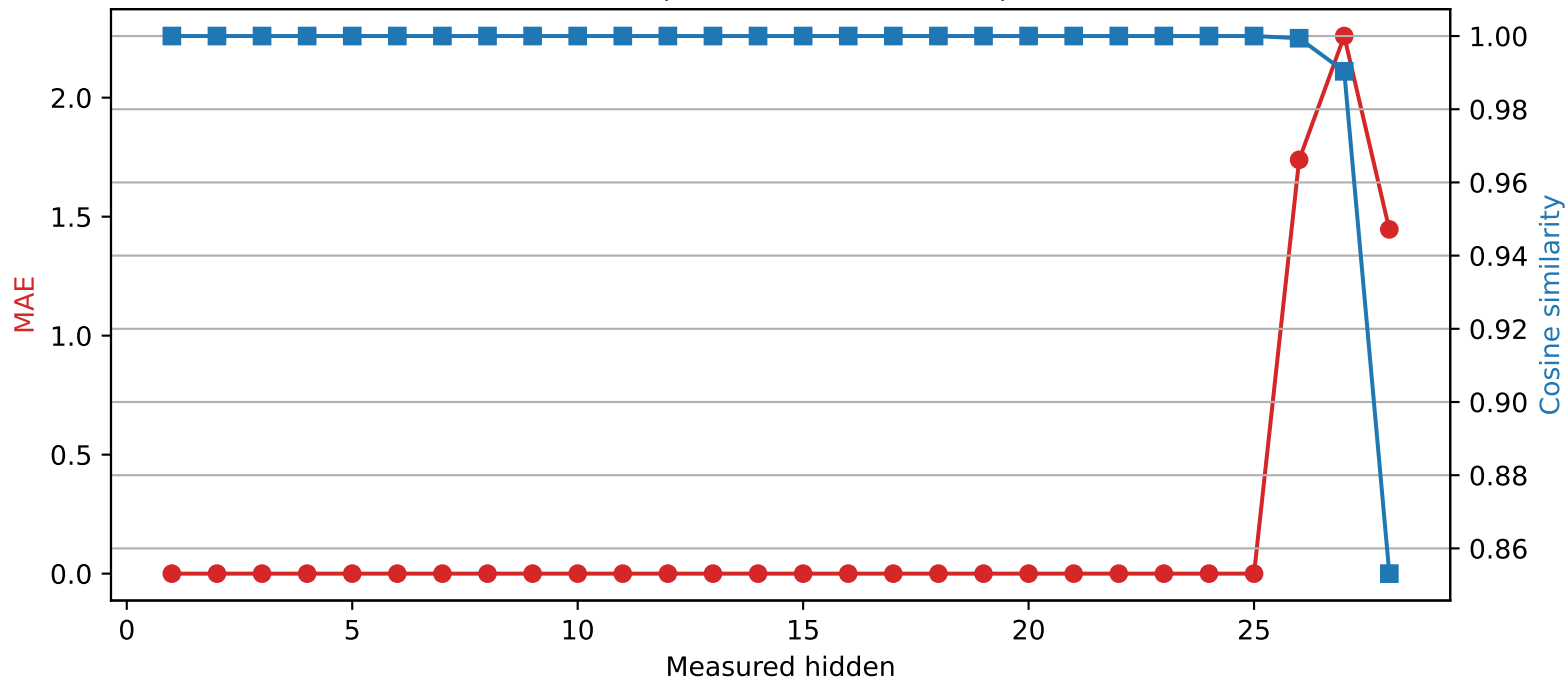
Qwen2.5-7B-Instruct | Quantized layer 25 | float16 \rightarrow int2
