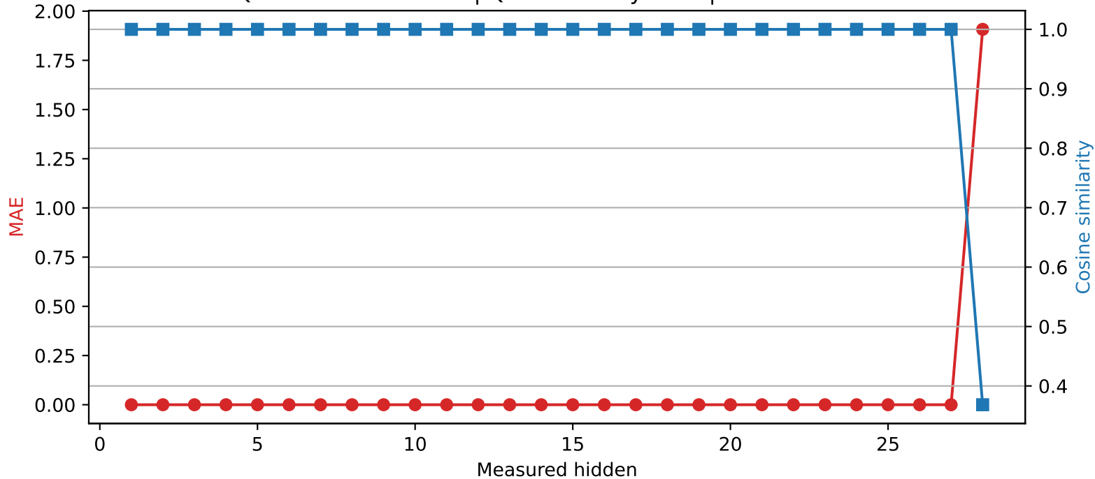
Qwen2.5-7B-Instruct | Quantized layer 27 | float16 → int2
