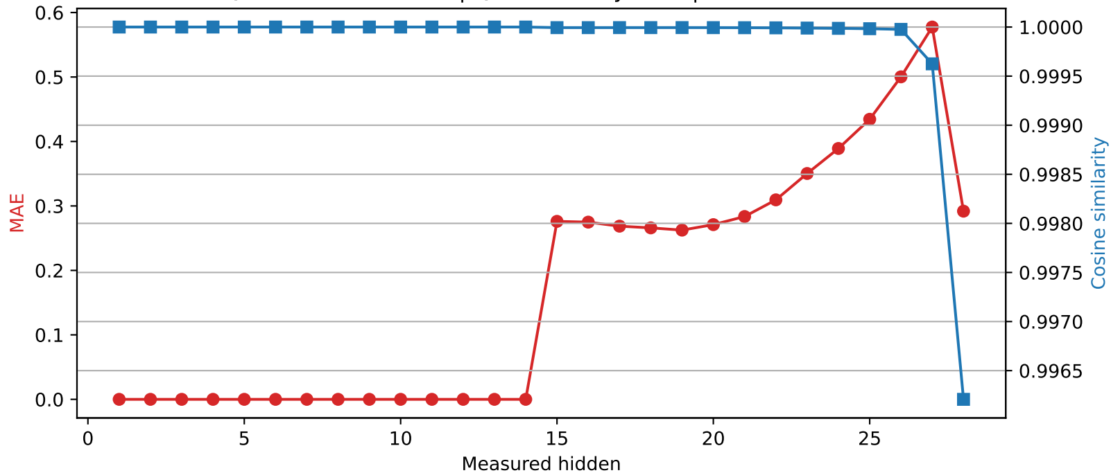
Qwen2.5-7B-Instruct | Quantized layer 14 | float16 → int2
