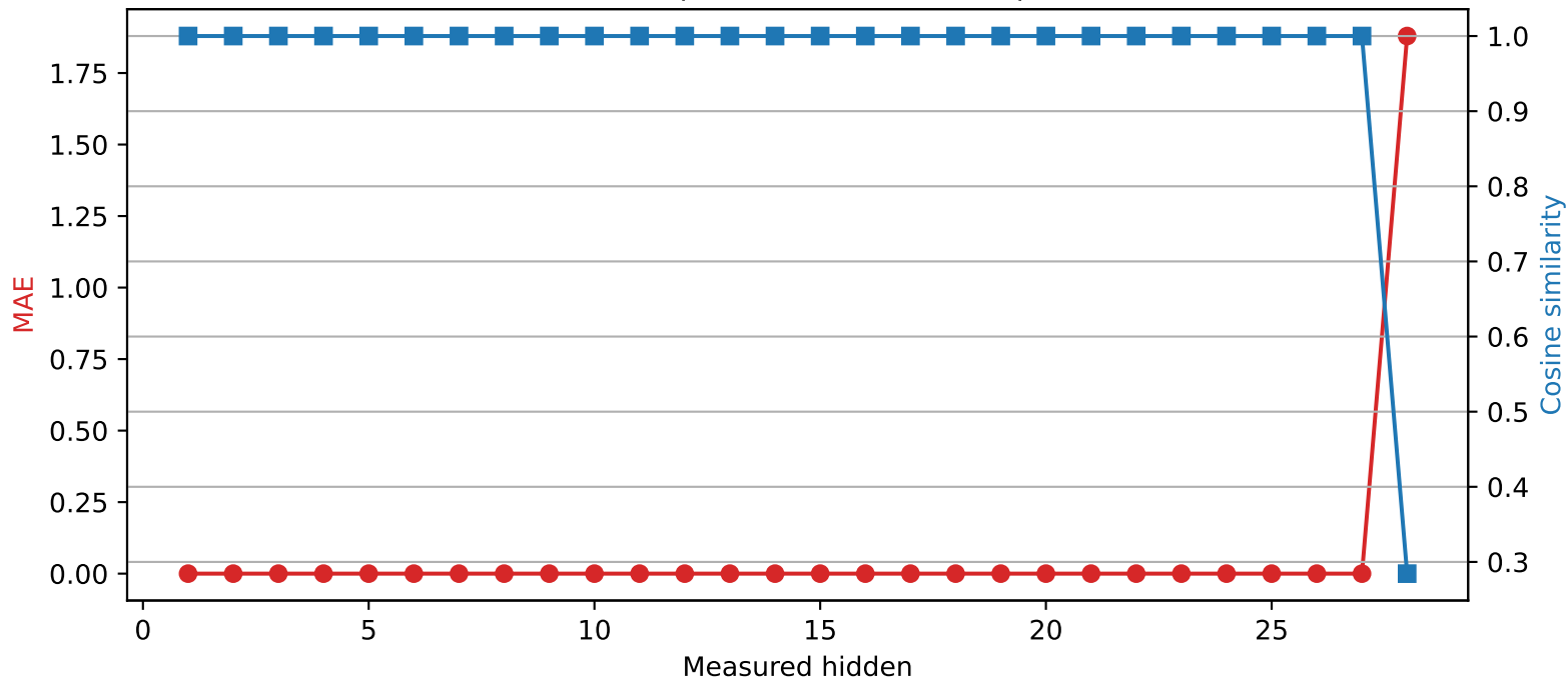
Qwen2.5-7B-Instruct | Quantized layer 27 | float16 \rightarrow int2
