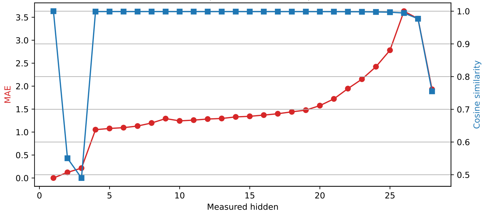
Qwen2.5-7B-Instruct | Quantized layer 1 | float32 → int2
