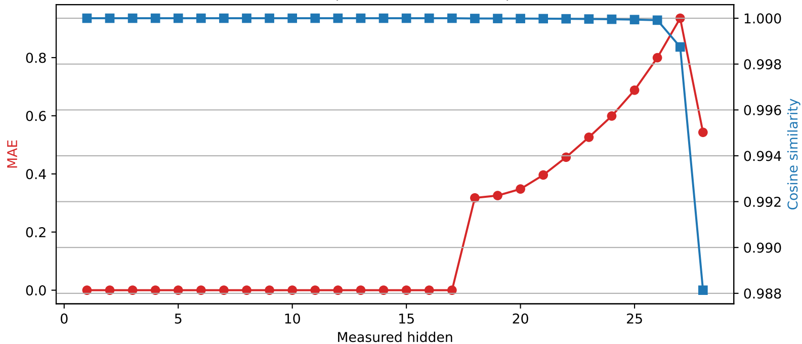
Qwen2.5-7B-Instruct | Quantized layer 17 | float32 → int2
