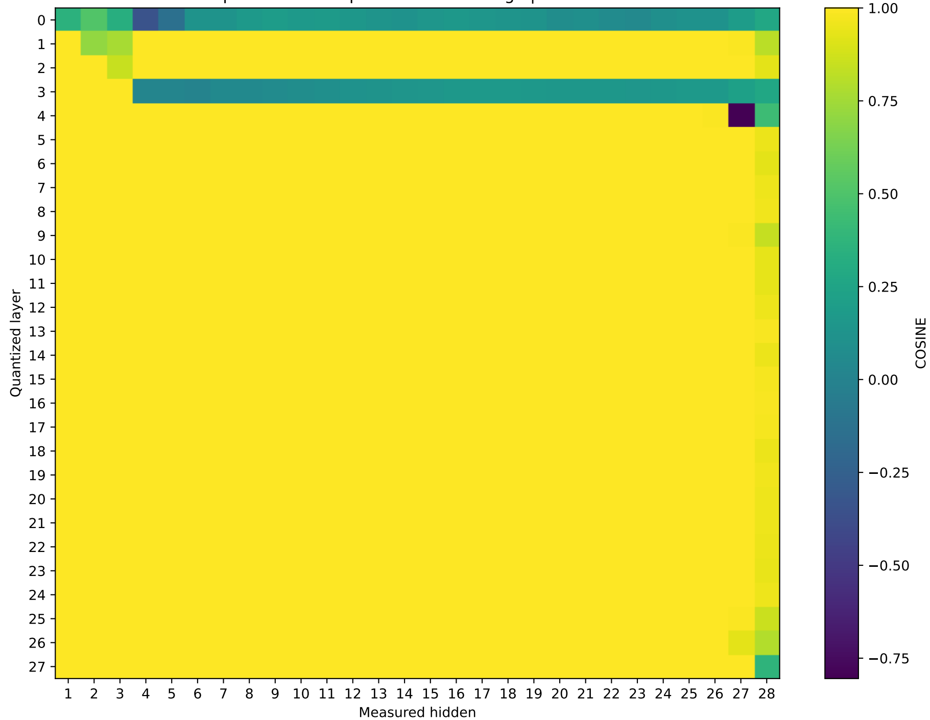
Qwen2.5-7B-Instruct Prompt 3: cos sim representation damage | float32 → int2
