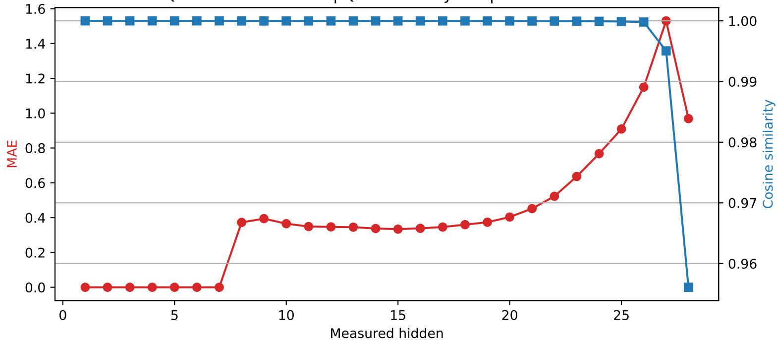
Qwen2.5-7B-Instruct | Quantized layer 7 | float32 \rightarrow int2
